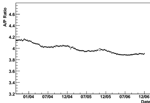
Figure 4: Area-to-peak ratio as a function of time for a typical PMT channel.
