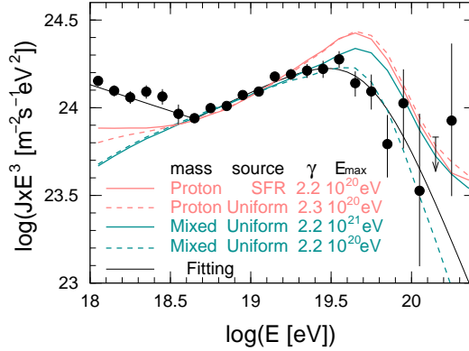
Figure 3: The combined energy spectrum multiplied by E^3 [15], together with a fit to Eq. 1 (black line), and the predictions of two astrophysical models (blue and red lines). The input assumptions of the models (mass composition at the sources, the source distribution, spectral index and exponential cutoff energy per nucleon at the acceleration site) are indicated in the figure.
