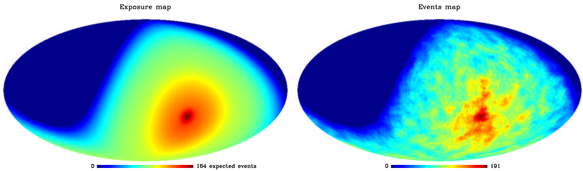
Figure 1. Left: semi-analytic Auger south sky coverage in the energy range [1-5] EeV. Right: real event map. The two sky maps are in galactic coordinates.
